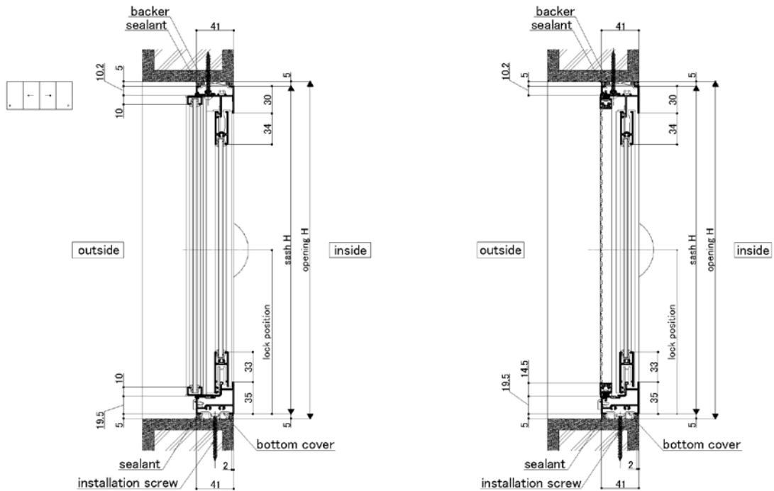
Vertical cross-section
