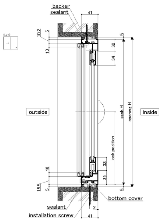
Vertical cross-section
